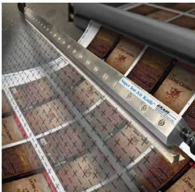
The Model 111048 48" (1219mm) Super Ion Air Knife neutralizes the static electricity and cleans the surface of the paper.
