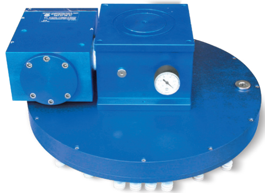
mm Ø400 with fixing support and vacuum interception solenoid valve - SO DO 40 V
