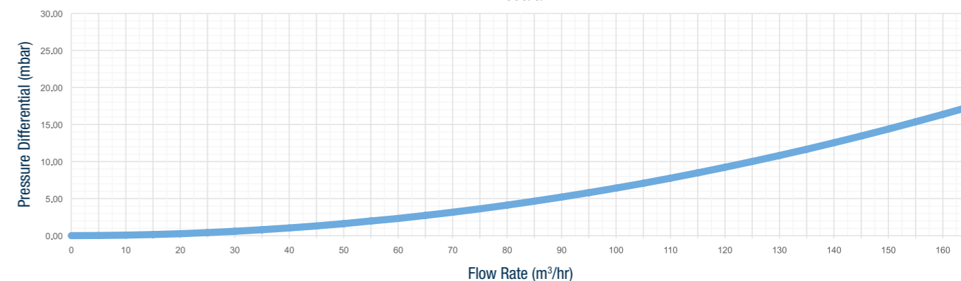
8" BoilermagXT BMXT300/8/AAV
