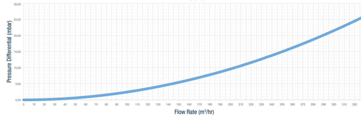
12" BoilermagXT BMXT400/12/AAV
