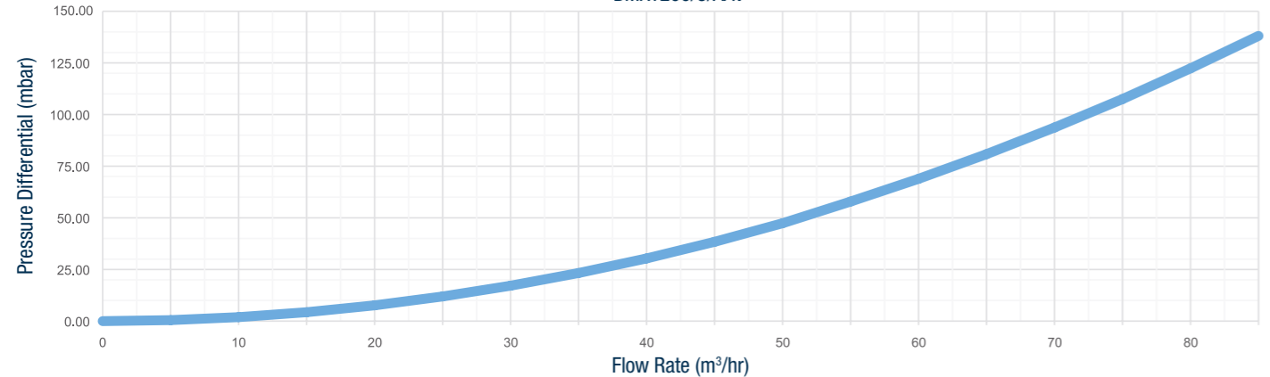
4" BoilermagXT BMXT200/4/AAV
