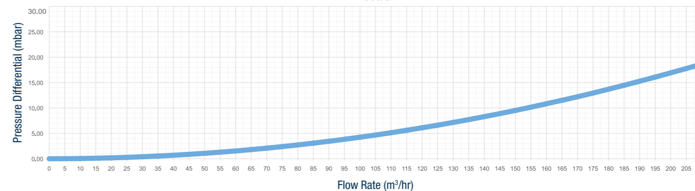
10" BoilermagXT BMXT400/10/AAV
