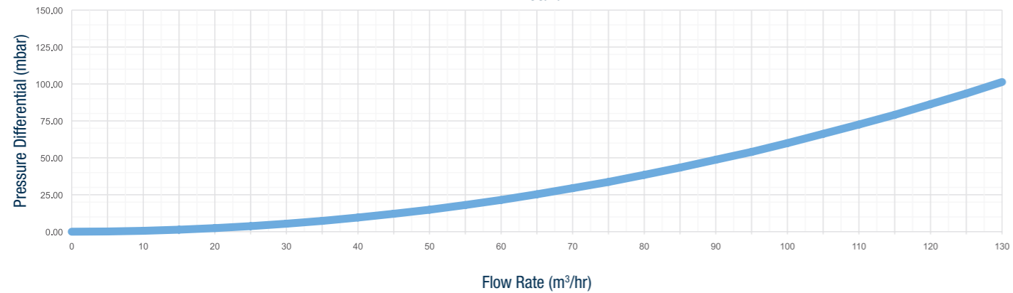
4" BoilermagXT BMXT200/4/AAV
