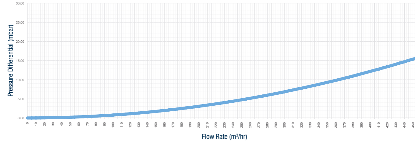
12" BoilermagXT BMXT400/12/AAV
