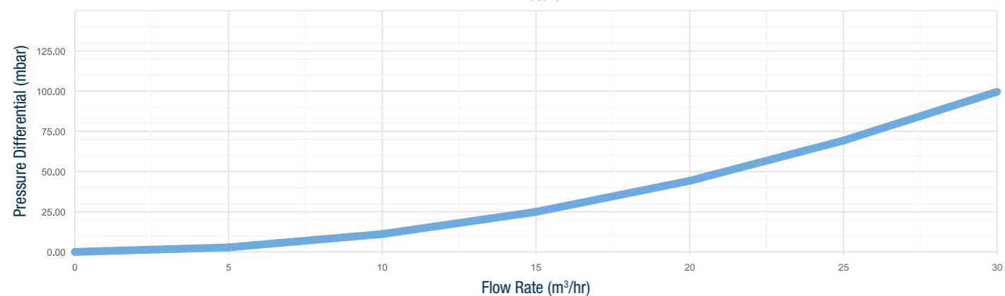
3" BoilermagXT BMXT200/3/AAV
