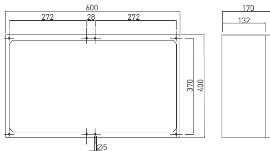
DIMENSIONS MCS 64/128 outlets (mm)
