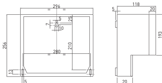
DIMENSIONS MCS 4 to 32 outlets (mm)
